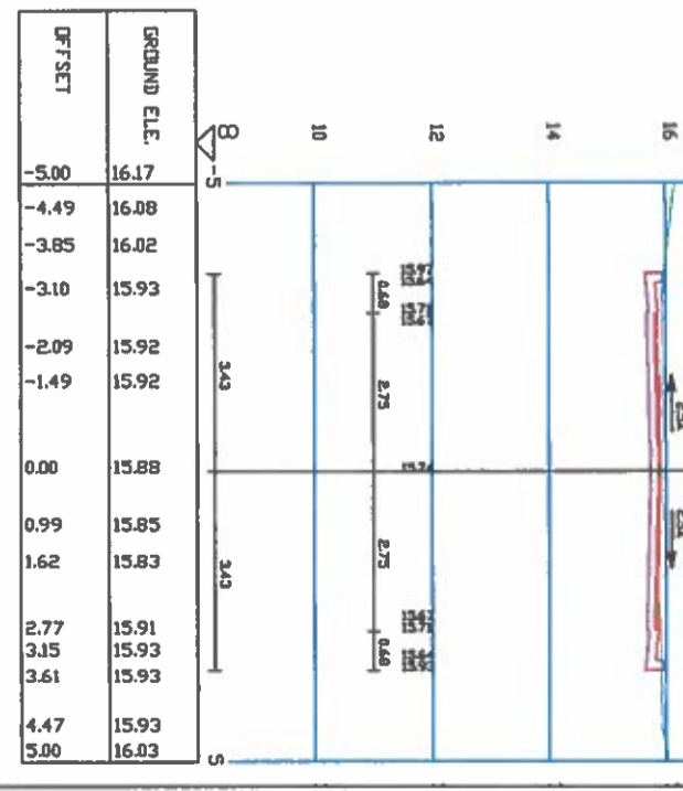
SECTION 0+325 St. 325 Berzelor
