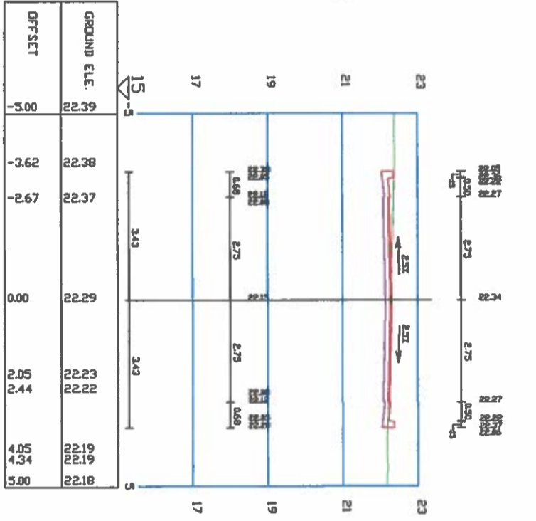
SECTION 0+250 St. 250 Berzelor
