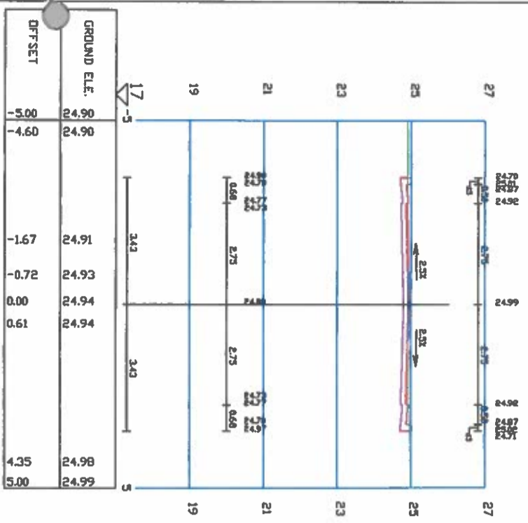
SECTION 0+200 St. 200 Berzelor
